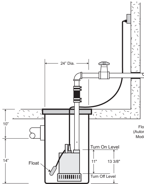
Typical Installation Automatic Models
