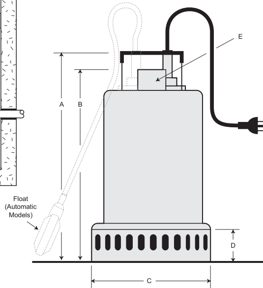
Dimensions For Automatic & Manual Models
