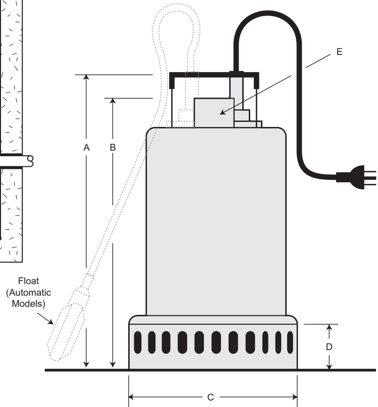
Dimensions For Automatic & Manual Models
