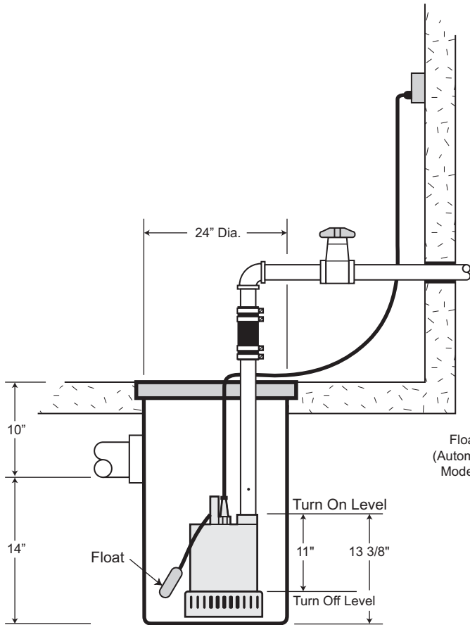
Typical Installation Automatic Models
